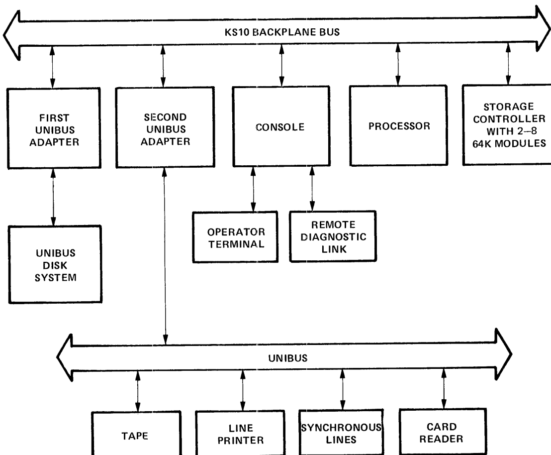
Figure 1.4: DECSYSTEM-2020
