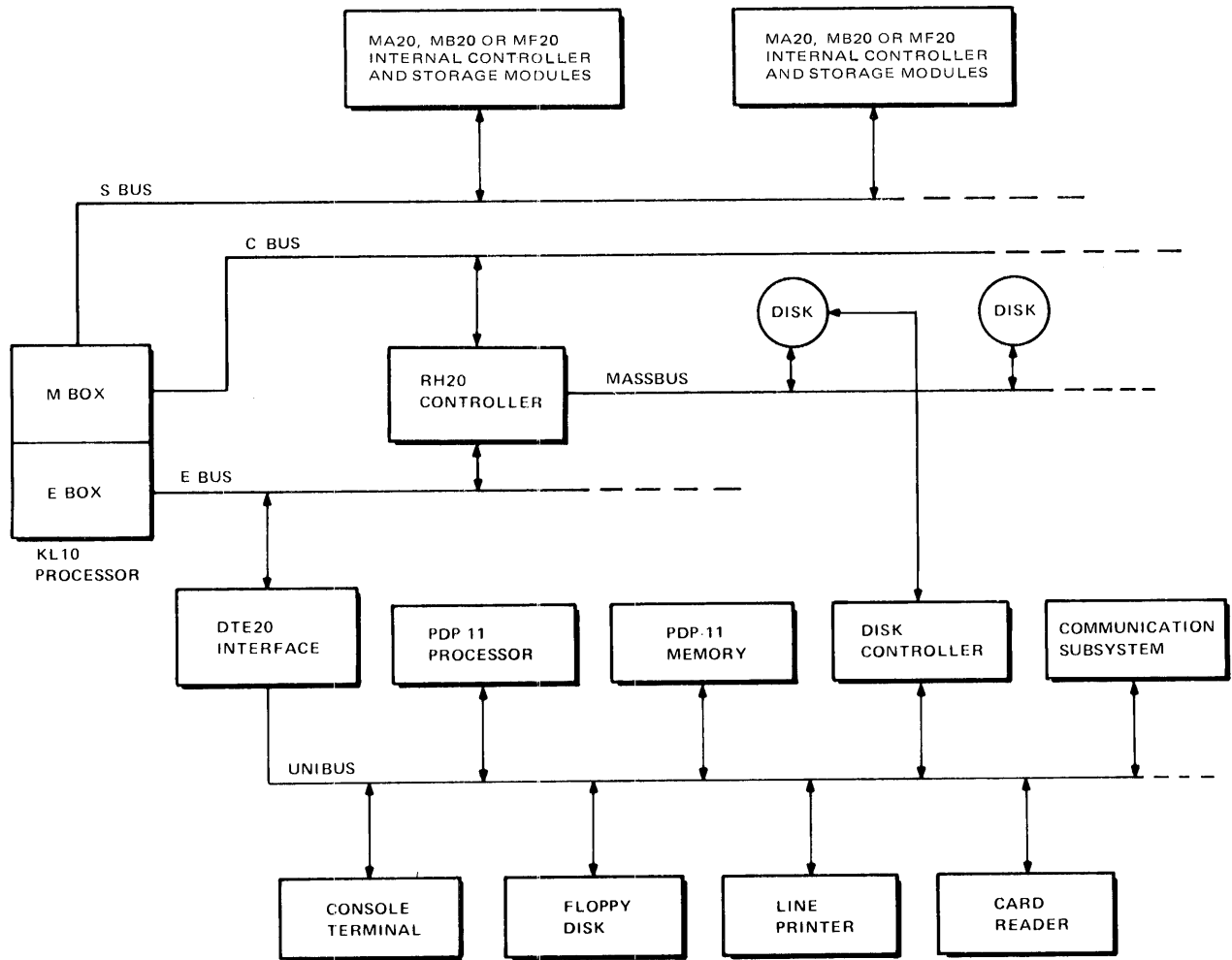
Figure 1.1: KL10-based DECSYSTEM-20
