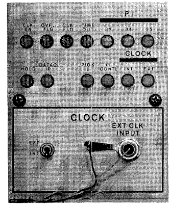
Clock Control Panel
